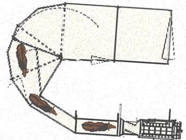
210 Sweep System with Eliminator Gate
